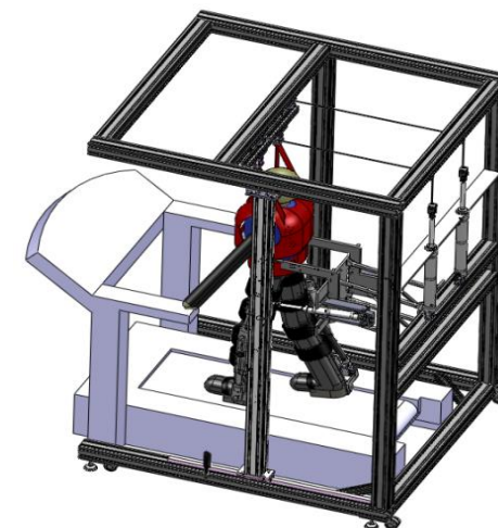
Exoskeleton-type gait rehabilitation robot
